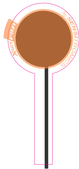
LOWER CIRCUIT (TOP SIDE) 1. CI-1001 CONDUCTIVE SILVER, 2. OVERPRINTED WITH DB-29 FSR #1 (EXCEPT TAIL)
