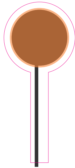
UPPER CIRCUIT (SUB SURFACE) 1. CI-1001 CONDUCTIVE SILVER, 2. OVERPRINTED WITH DB-29 FSR #1 (EXCEPT TAIL)
